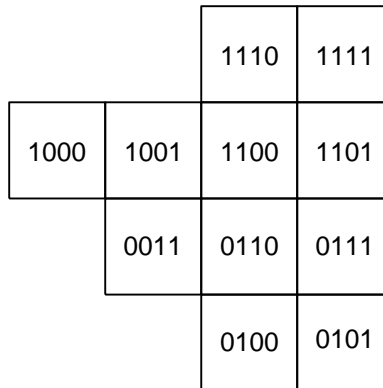
Figure 20: Morton Ordering in an Irregular Grid
