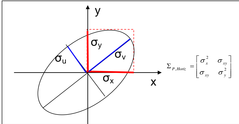
Figure 28: Horizontal Error Ellipse at a Point
