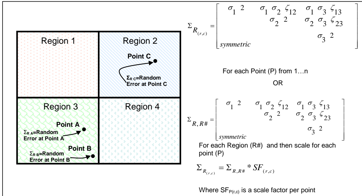
Figure 23: The Random Error ( \Sigma_R ) at a Point (P)
