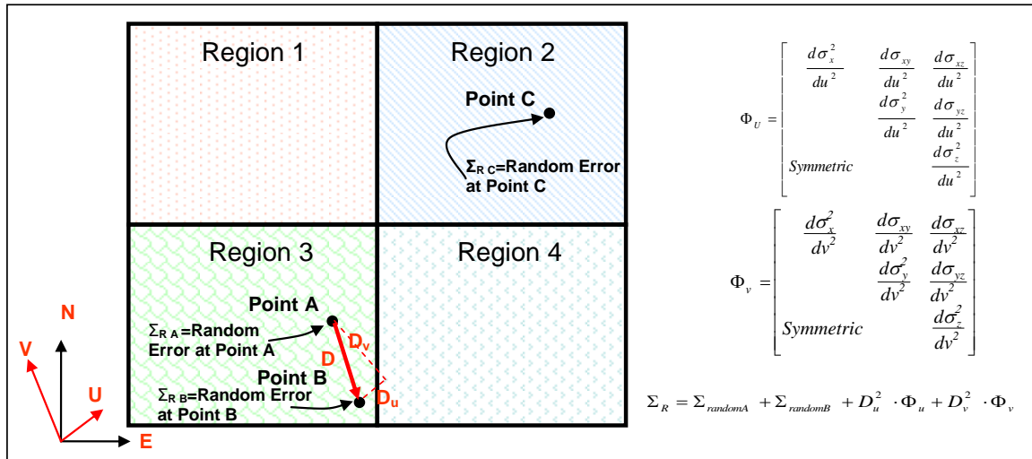
Figure 24: Relative Covariance of Vector R within a Region
