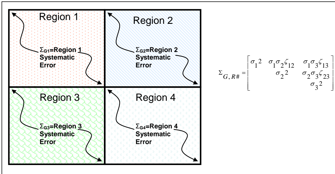
Figure 22: Systematic Error ( \Sigma_{G,R\#} ) per Region
