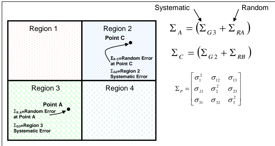
Figure 27: Covariance Data at a Point
