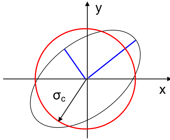
Figure 29: Circular Error from Covariance Data
