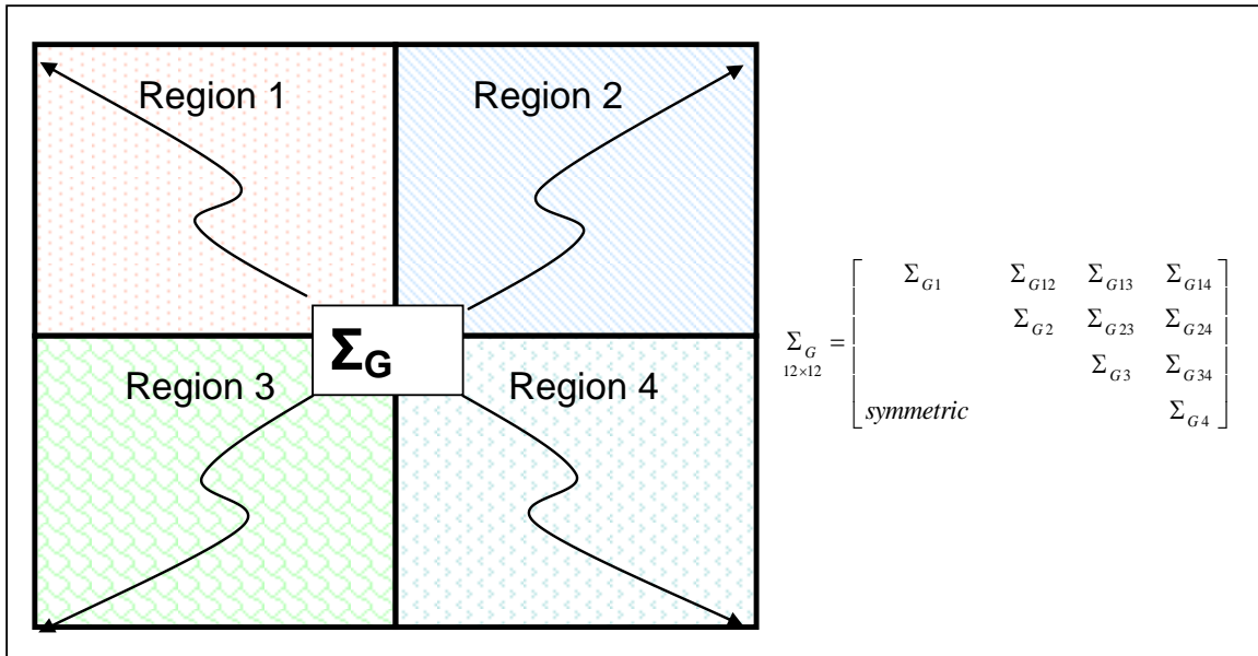
Figure 21: Full Covariance Data for the Systematic Errors of Four Regions
