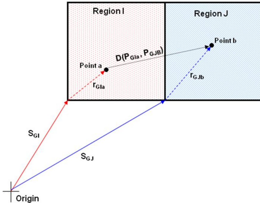
Figure 25: Systematic and Random Error Vector Representation
