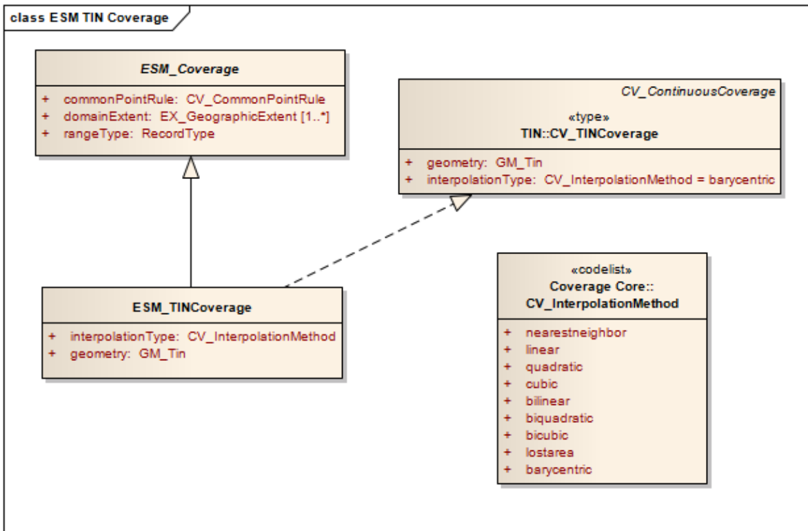
Figure 8: ESM TIN Coverage
