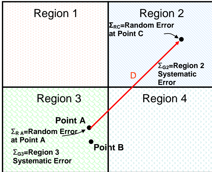
Figure 26: Sample DEM Footprint Consisting of Four Regions with Vector Crossing Regions
