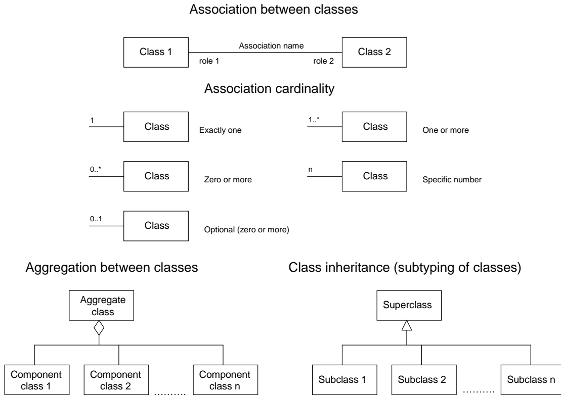
Figure 18: UML Class Relationships
