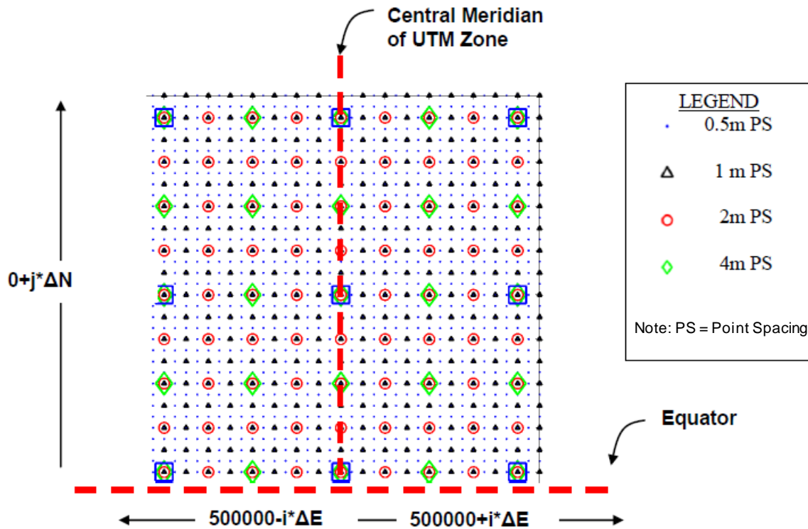
Figure 2: Example of UTM Point Location in Northern Hemisphere
