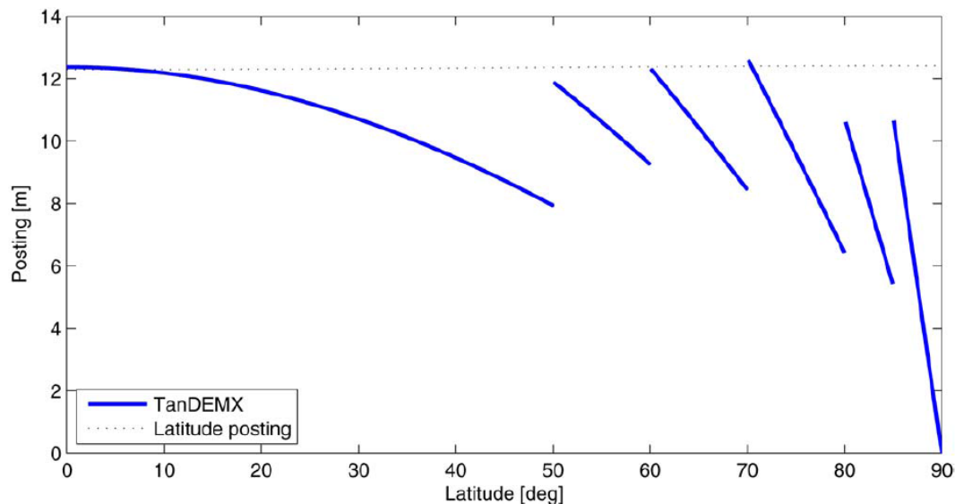
Figure 4: Longitudinal posting as a function of latitude
