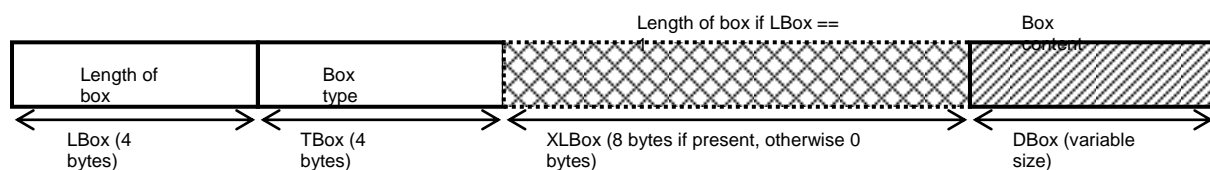
Figure 2 – JPEG 2000 box structure
