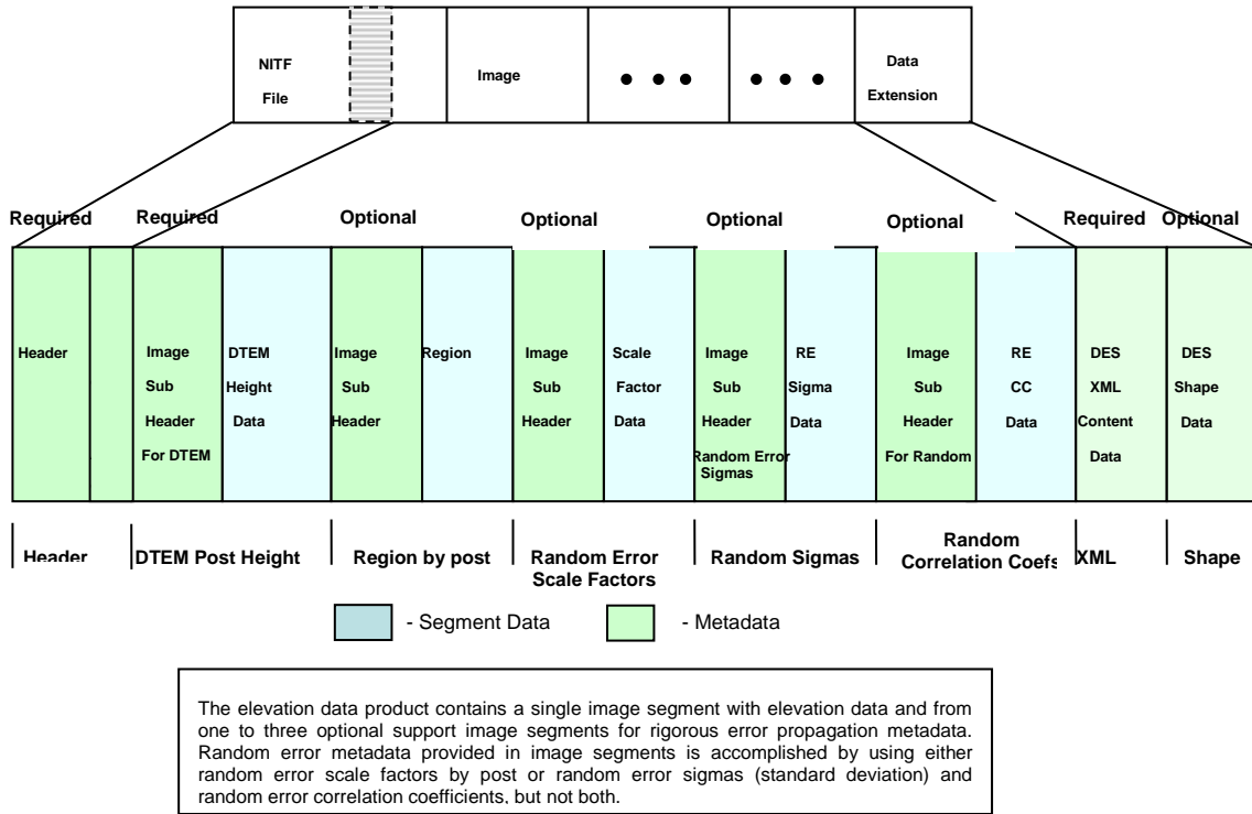
Figure B-1 Diagram showing NSIF/NITF File Format
