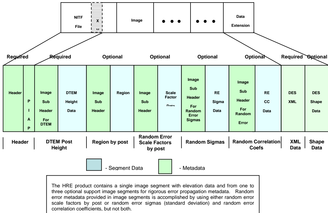
Figure 1: NSIF/NITF structure of an ESM based product (block format)
